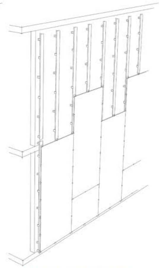
Vertical orthogonal modulation with locked joints
