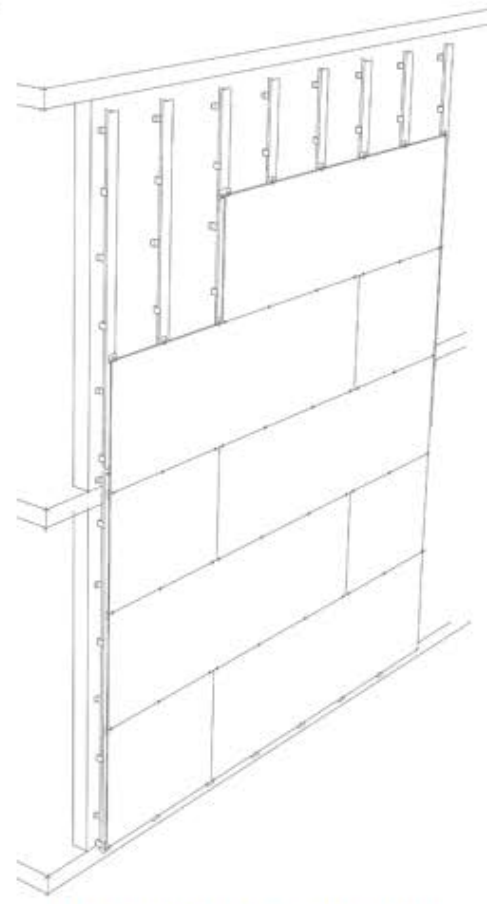
Horizontal orthogonal modulation with locked joints
