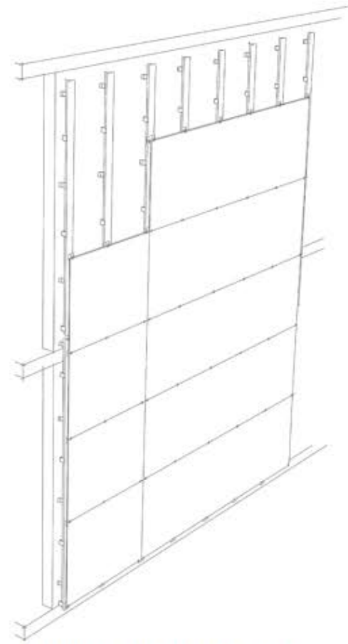
Horizontal orthogonal modulation with straight joints
