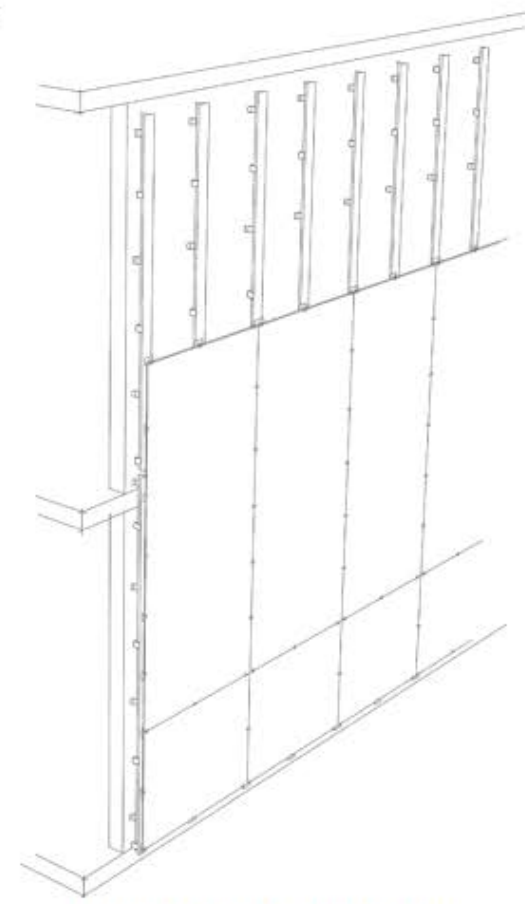
Vertical orthogonal modulation with straight joints
