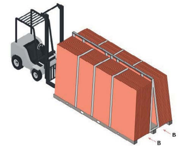
Forklift with 5000 kg Capacity to carry from direction A
